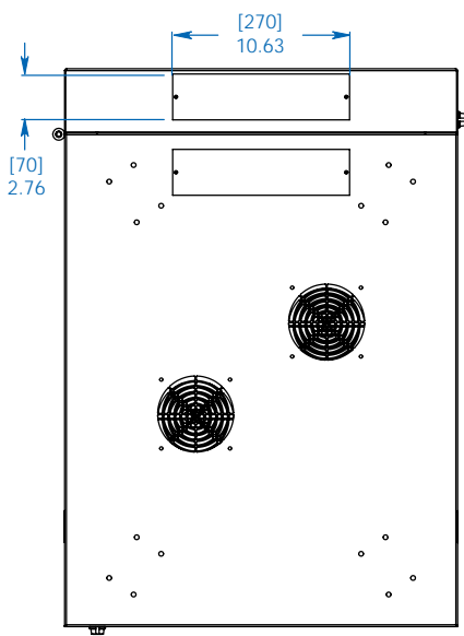
TOP/BOTTOM VIEW
