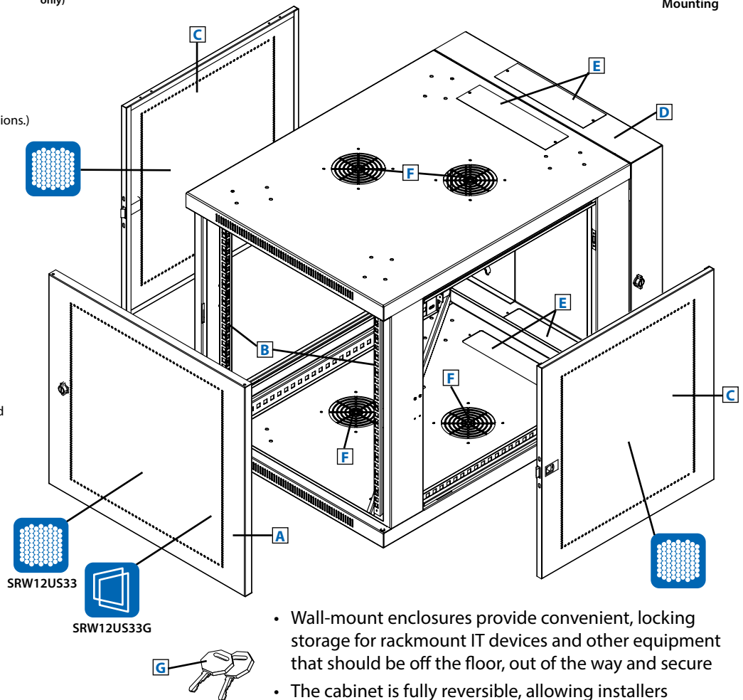
Floor-Standing Installation: Optional SRCASTER kit adapts cabinet to roll under desks, tables or counters. (Kit includes 4 casters.)
